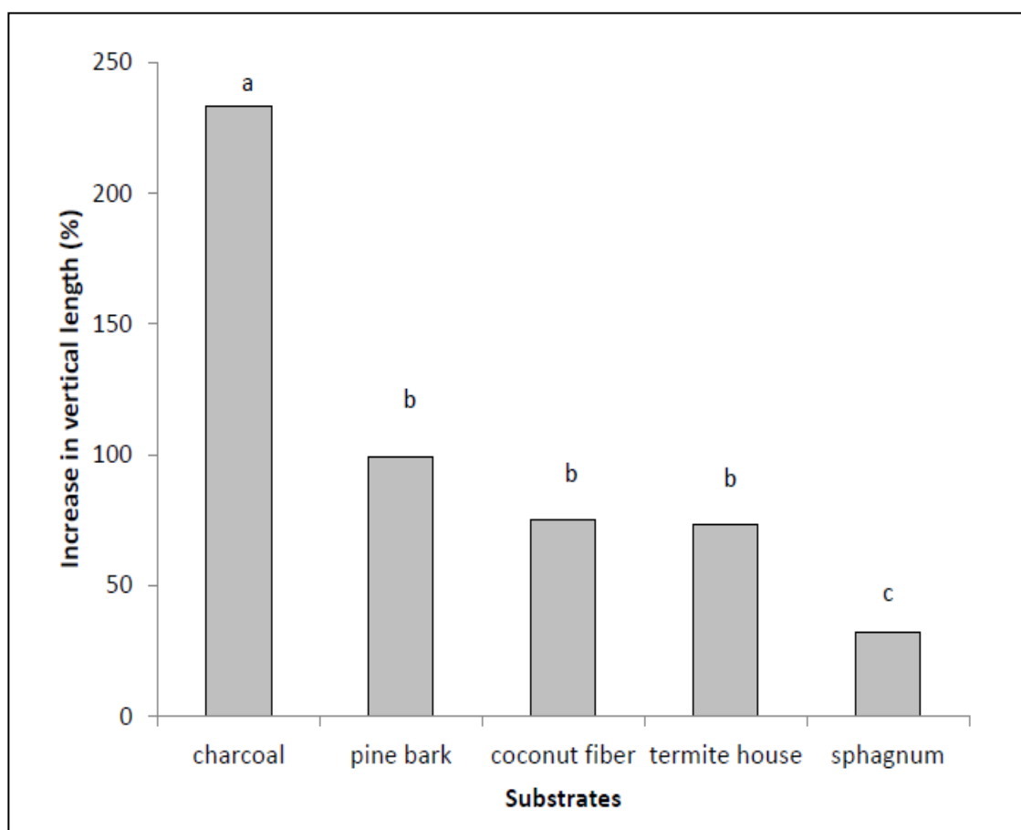
Figure 1 - Percentages of increase in vertical length in Epidendrum ibaguense plantlets after 60 days of acclimatization in different substrates. Letters indicate difference by Tukey test at a 5% level.
