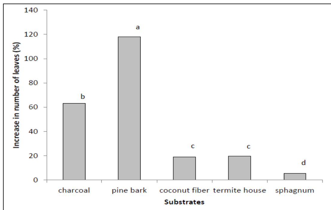
Figure 2 - Percentages of increase in number of leaves in Epidendrum ibaguense plantlets after 60 days of acclimatization in different substrates. Letters indicate difference by Tukey test at a 5% level.
